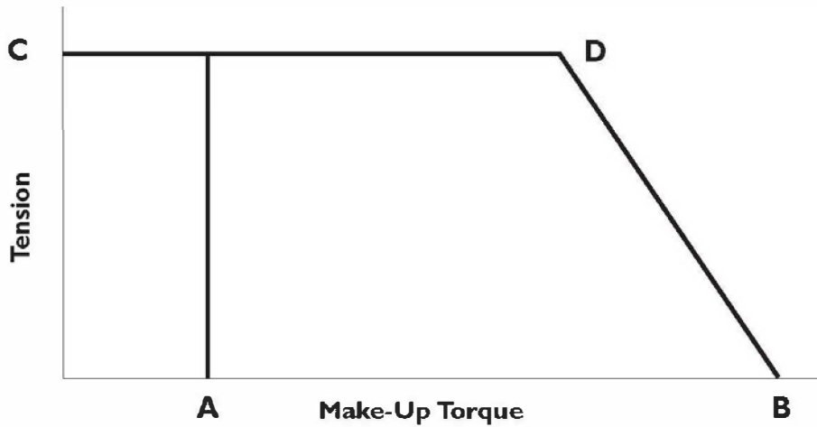
Tension Versus Make-Up Torque
